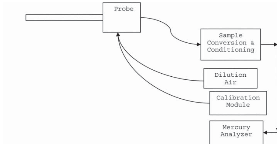
FIGURE A-1. TYPICAL MERCURY CEMS
